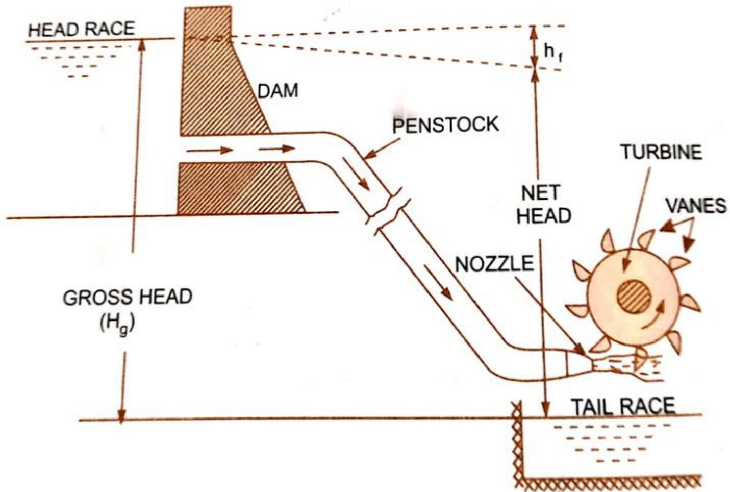
Fig. Layout of a hydroelectric power plant.
